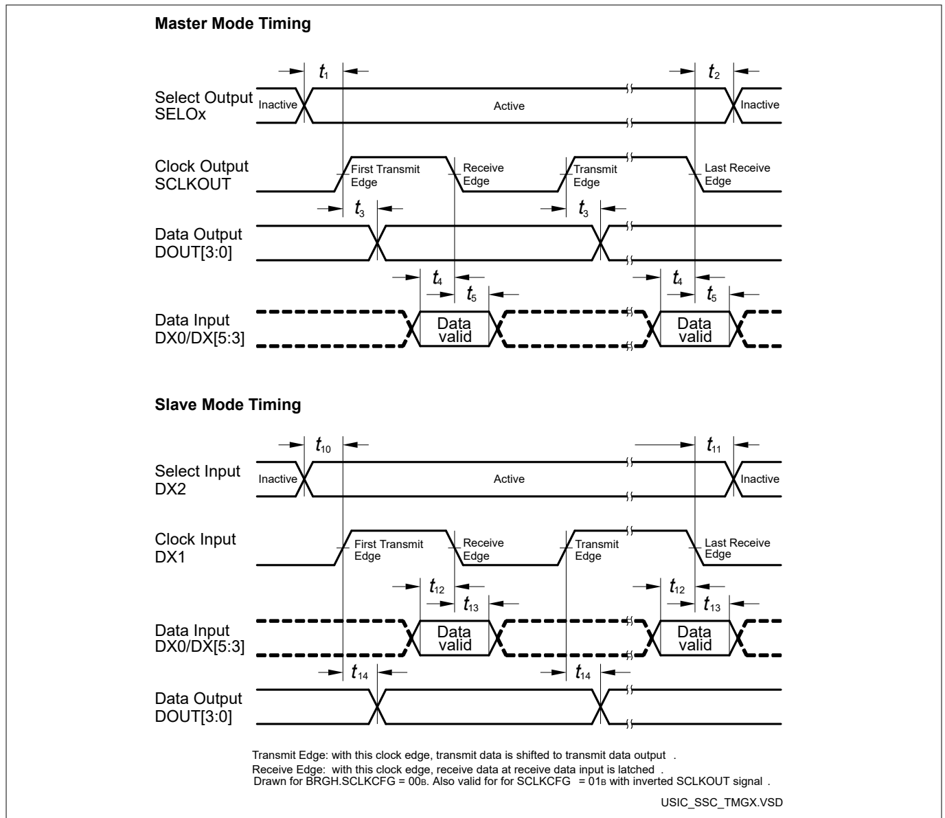
Figure 34 USIC - SSC Master/Slave Mode Timing
