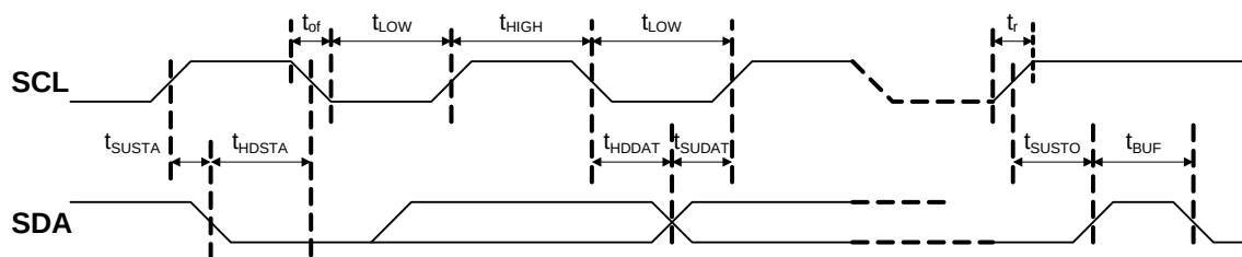
Figure 15. I²C / SMBus Timing
