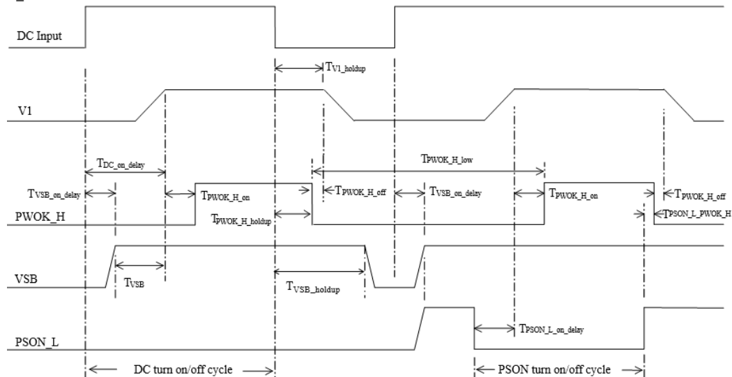
Figure 13. Turn On/Off Timing
