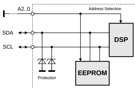
Figure 16. I²C Bus to DSP and EEPROM
