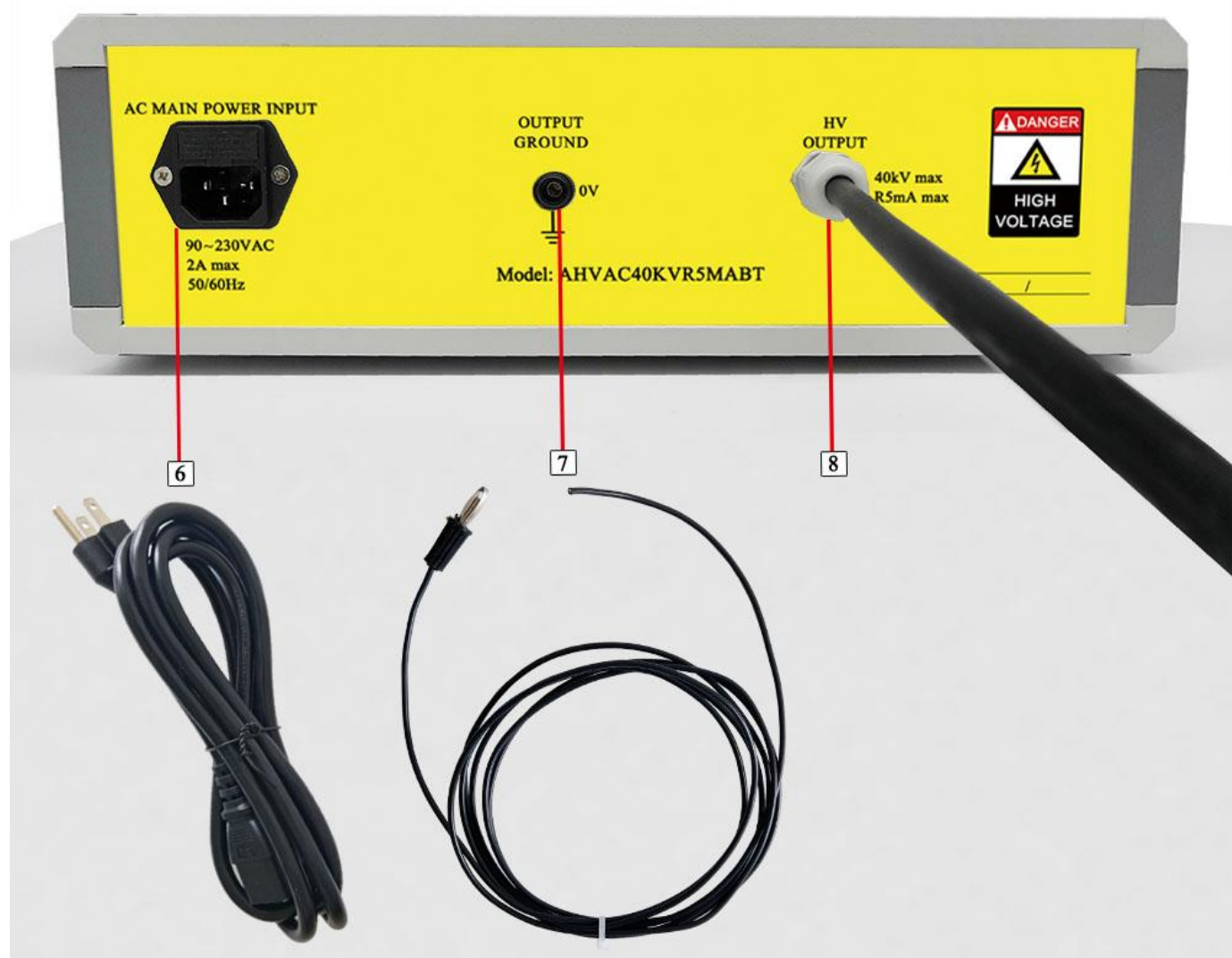
Figure 3. Back Panel
