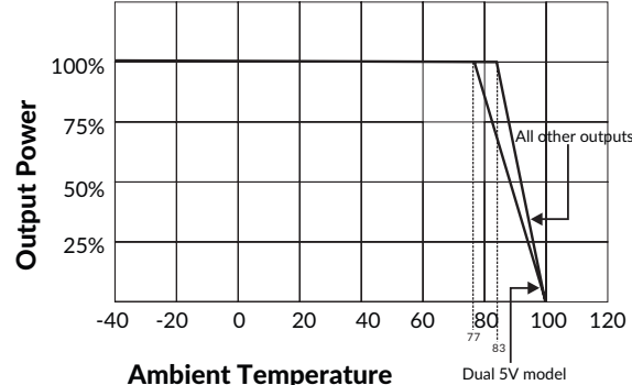
With heatsink
