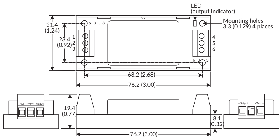
Chassis Mount with Heatsink -HK
