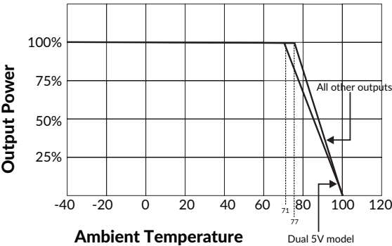
Without heatsink
