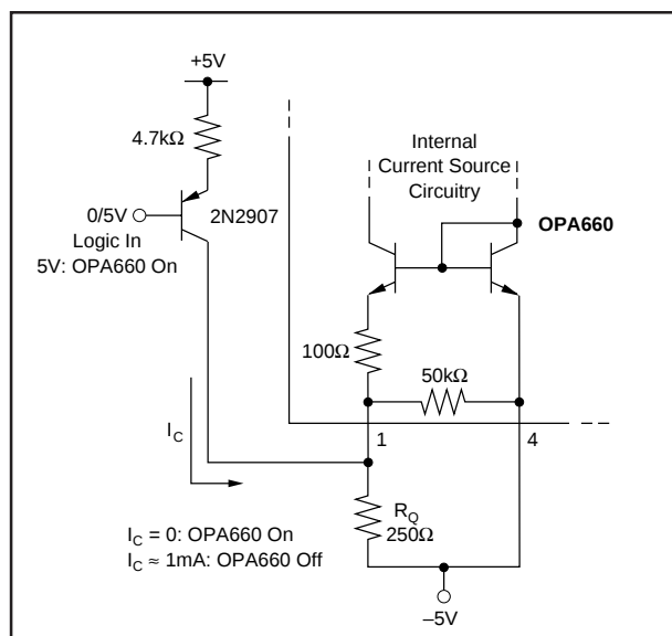
FIGURE 4. Logic-Controlled Disable Circuit.
