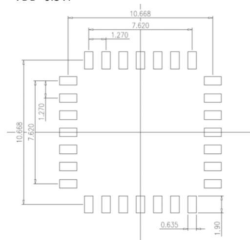
Figure 15: Recommended Pad Layout in mm (top view)
