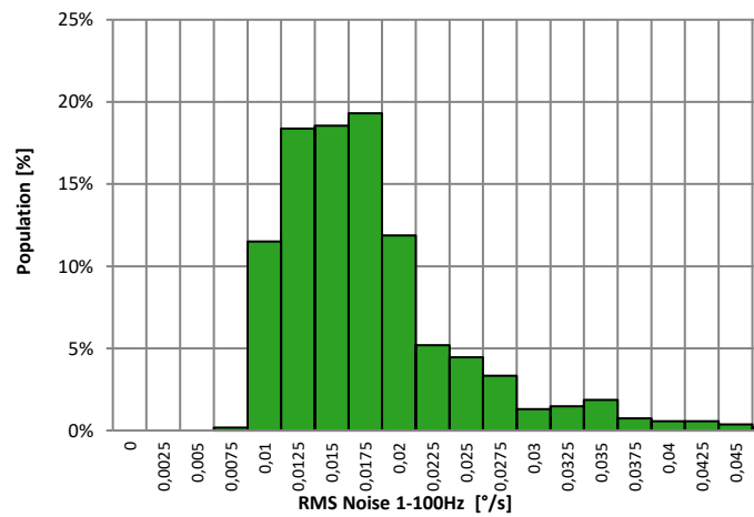
Figure 8: Distribution of RMS Noise in [1 -100Hz] band
