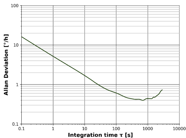
Figure 7: Allan variance (at 35°C)
