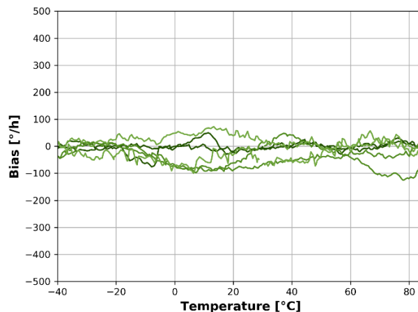
Figure 5: Residual bias temperature error (3 samples)
