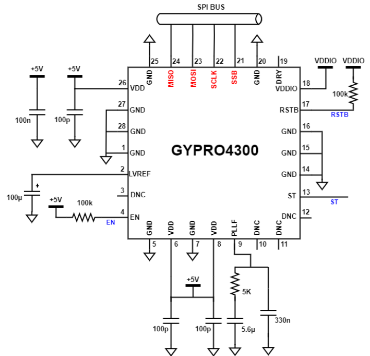
Figure 14: Recommended Application Schematic
