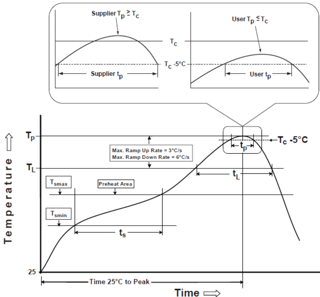
Figure 16: Recommended Reflow Profile, according to IPC/JEDEC J-STD-020D.1
