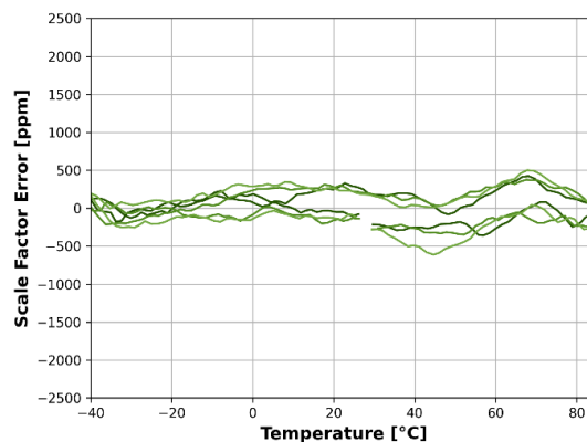
Figure 6: Residual scale factor error (3 samples)
