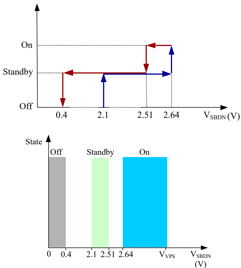
Figure 3. V_{SBDN} vs. Amplifier States
