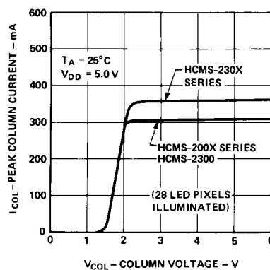
Figure 3. Peak Column Current vs Column Voltage
