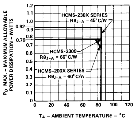
Figure 1. Maximum Allowable Power Dissipation vs Ambient Temperature as a Function of Thermal Resistance Junction-to-Ambient, R_{\theta JA} . Derated Operation Assumes R_{\theta PCA} = 35^{\circ}\text{C/W} Per Display for the Printed Circuit Board. T_J (IC) MAX = 125^{\circ}\text{C} .
