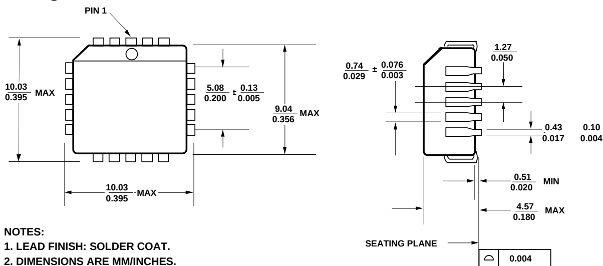
20 PIN PLASTIC LEADED CHIP CARRIER PACKAGE
